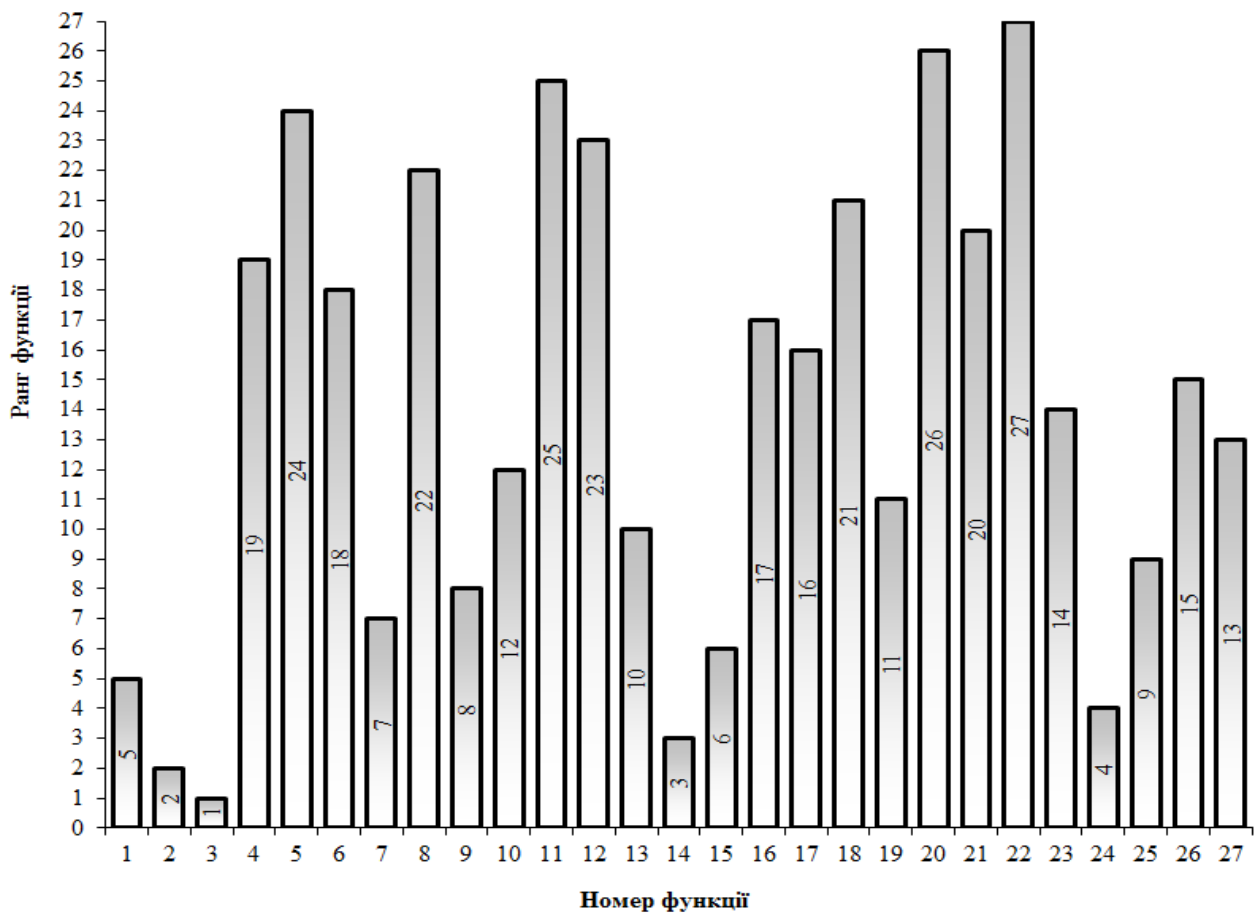
Fig. 10. Ranking diagram of blocks and mechanisms functions of Kalashnikov assault rifle relatively functional-cost index
