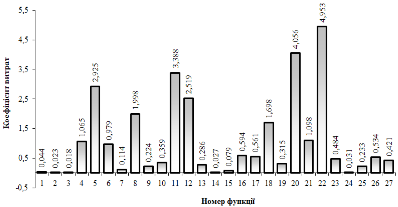
Fig. 7. Cost diagram of blocks and mechanisms functions of Kalashnikov assault rifle
