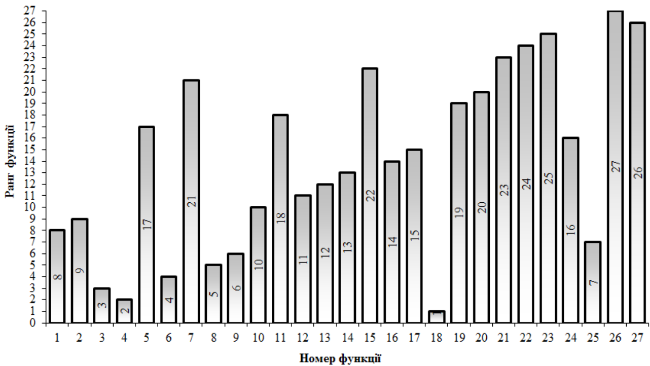
Fig. 5. Ranking diagram of blocks and mechanisms functions of Kalashnikov assault rifle relatively utility coefficient
