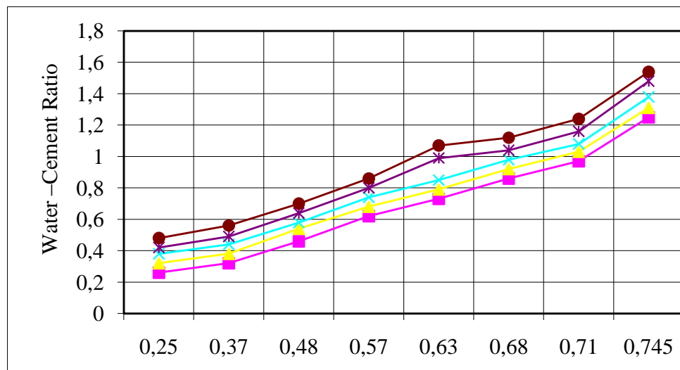
Fig. 1. Impact of the metal filler content on the water needs of the mixture samples: 1 – small cone spread on the shaker apparatus 101 – 108 mm; 2 – the same 112 – 122 mm; 3 – the same 126 – 133 mm; 4 – the same 144 – 149 mm; 5 – the same 158 – 169 mm
