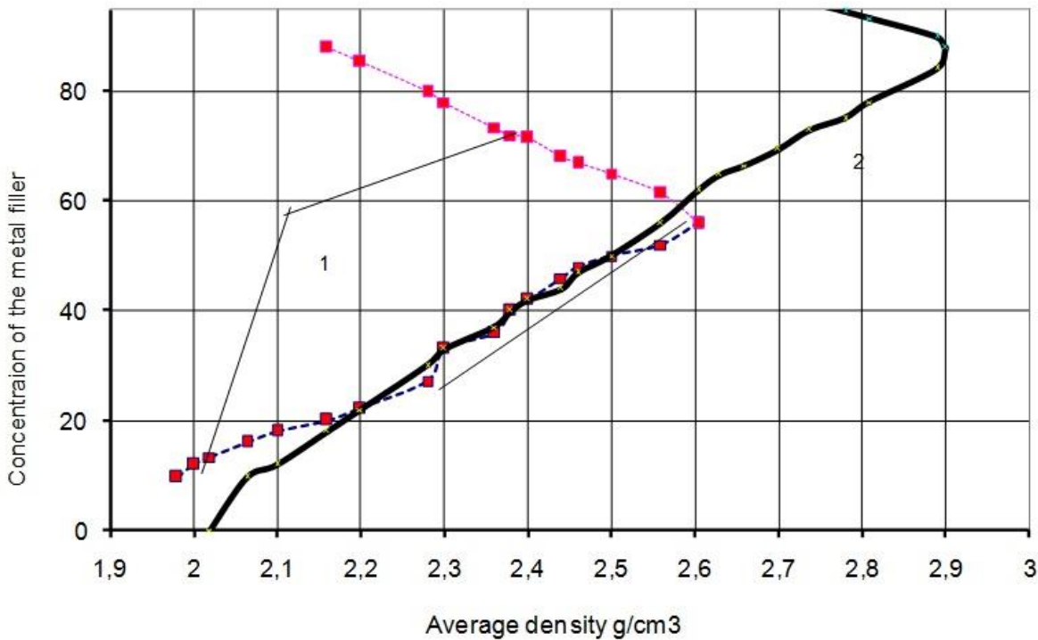
Fig. 3. Impact of the amount of the metal filler on the average density of the pressed tiles: 1 – metal-cement mixtures; 2 – the same with the addition of the coarse sand
